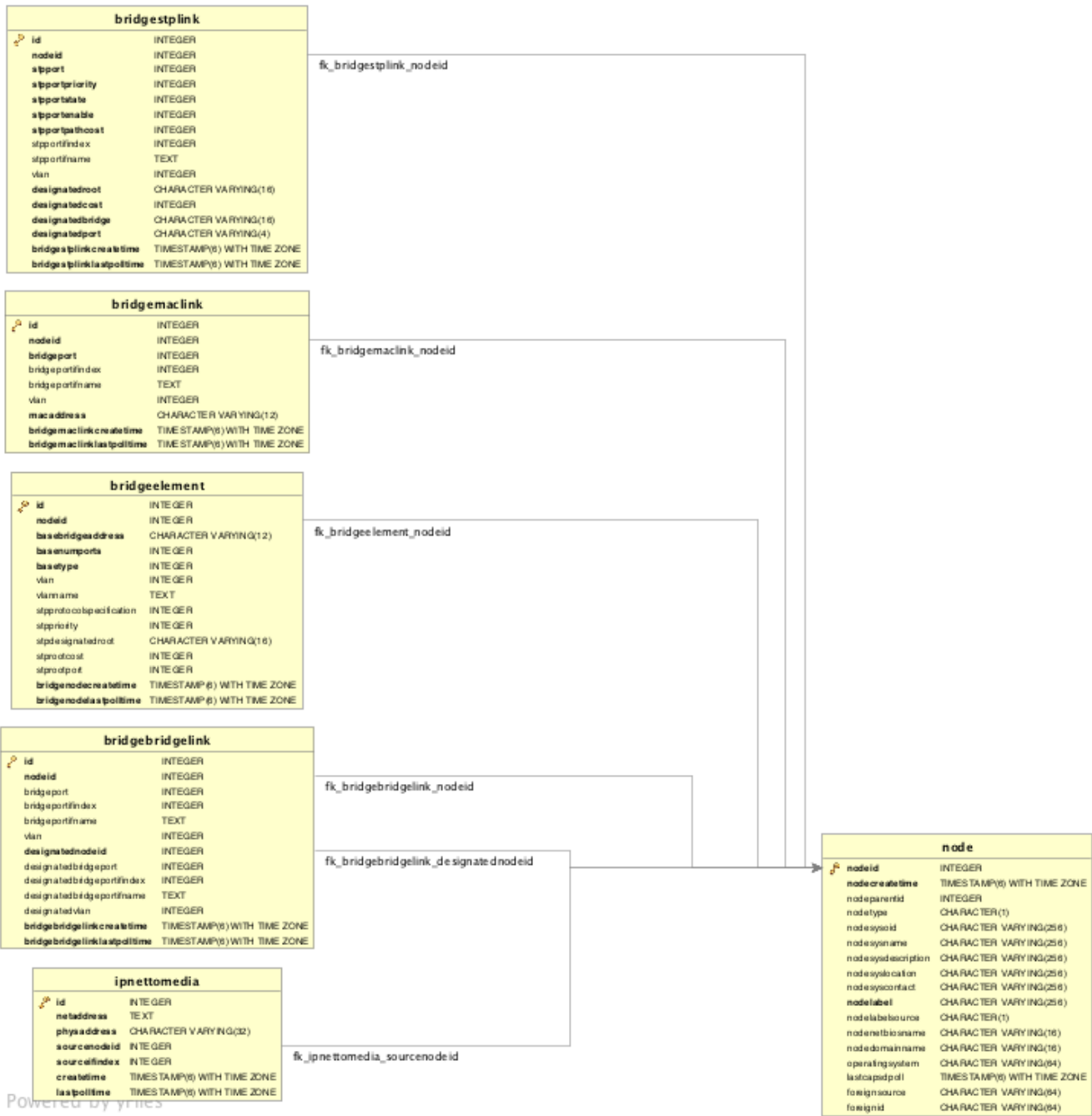
Figure 38. Database tables related to transparent bridge discovery
